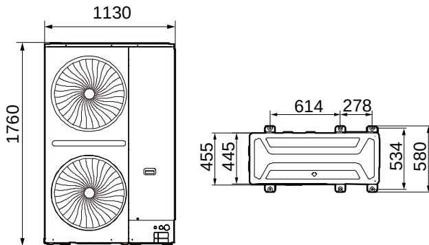
Figure 2-2.1: 8/10/12/14/16 HP dimensions (unit: mm)
