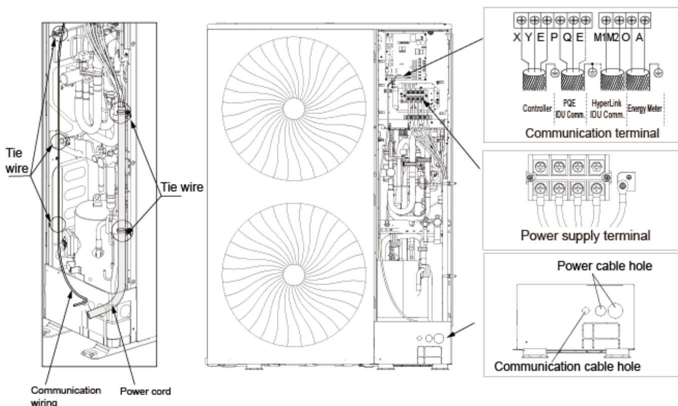
Figure 3-9.1: Wiring layout
