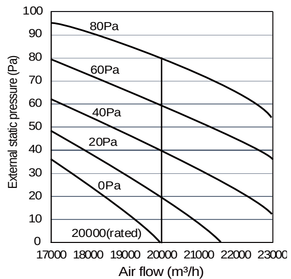
Figure 3-3.7: 18HP units fan performance
