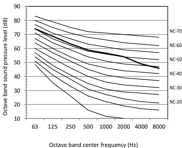
Figure 2-10.3: 16HP octave band level
