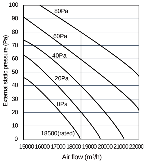
Figure 3-3.10: 24HP units fan performance
