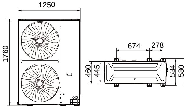
Figure 2-2.2: 18/20/22/24HP dimensions (unit: mm)
