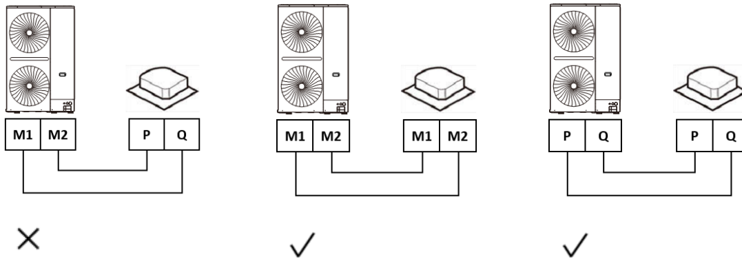
Figure 3-9.5: Communication wiring
