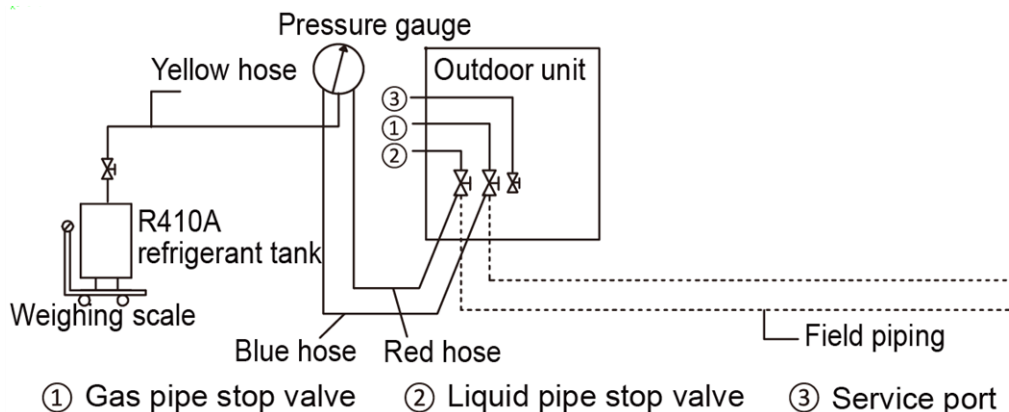
Figure 3-8.1: Charging refrigerant
