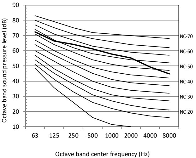
Figure 2-10.7: 24HP octave band level
