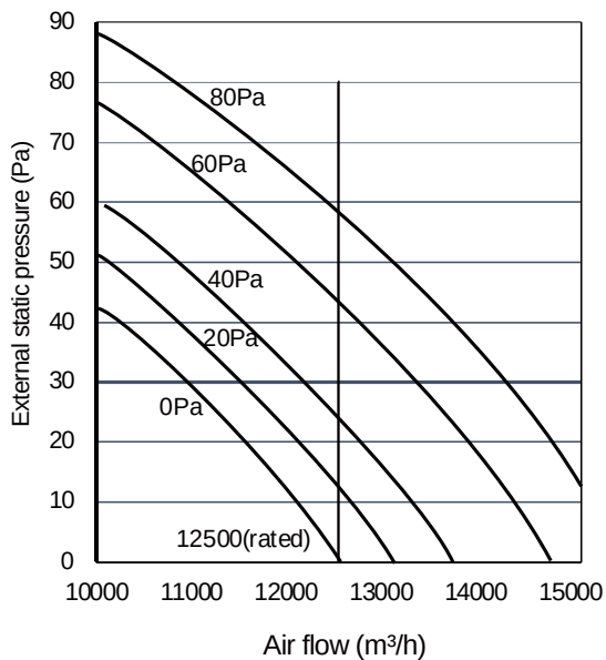
Figure 3-3.6: 16HP units fan performance
