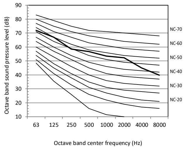
Figure 2-10.2: 14HP octave band level
