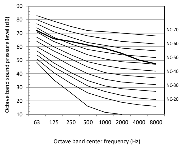
Figure 2-10.6: 22HP octave band level
