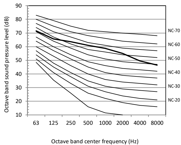
Figure 2-10.5: 20HP octave band level
