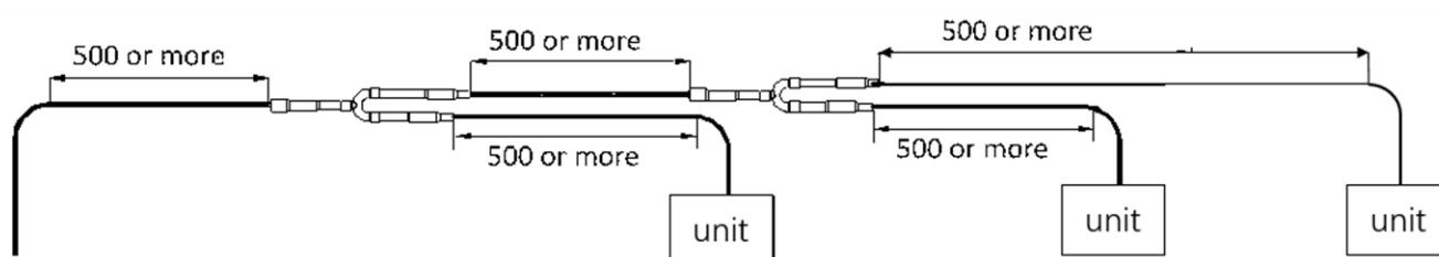
Figure 3-5.10: Branch joint spacing and separation from bends (unit: mm)
