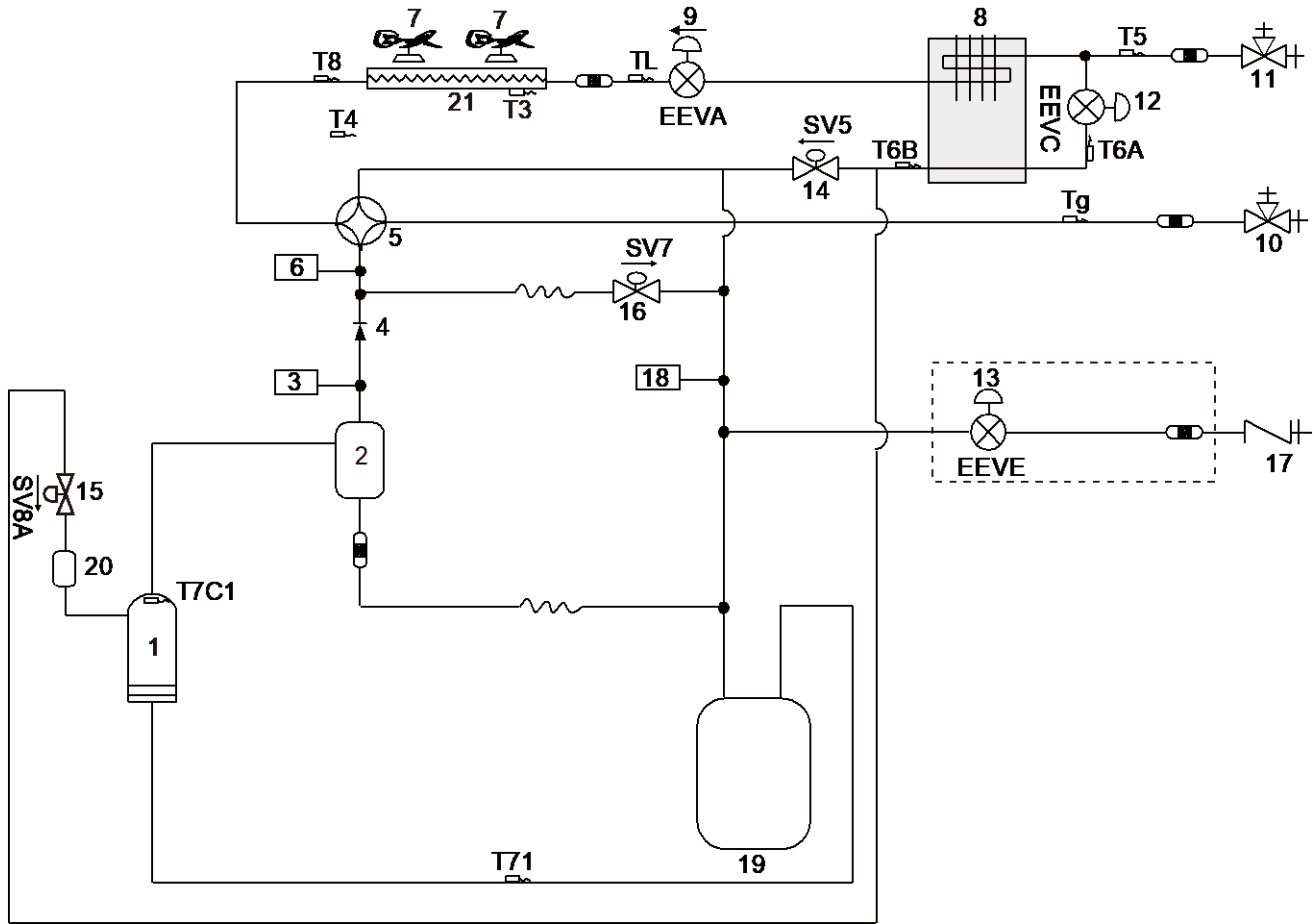
Figure 2-4.1: 8-16HP piping diagram
