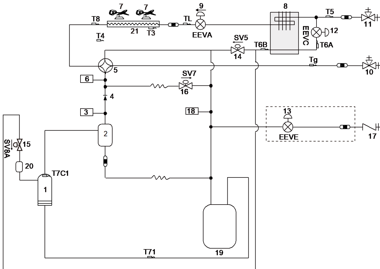
Figure 2-4.2: 18-24HP piping diagram
