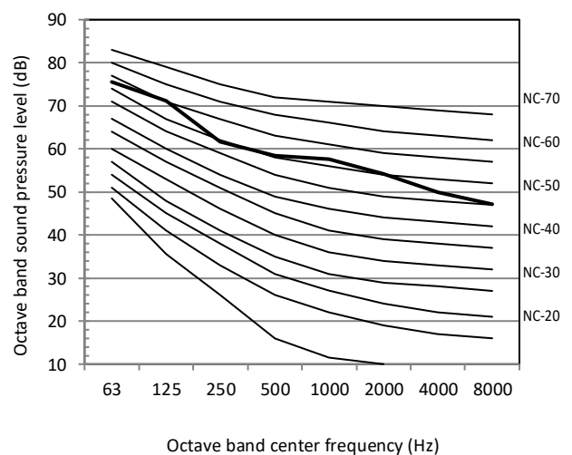
Figure 2-10.4: 18HP octave band level
