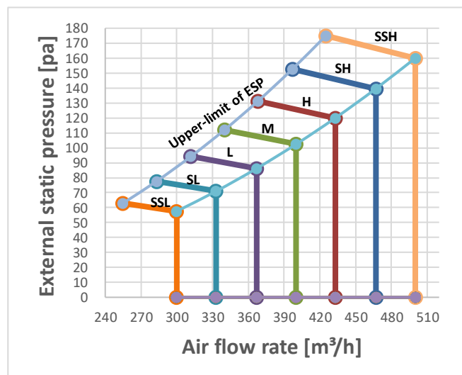
Figure 9.2: MIH22T2HN18
