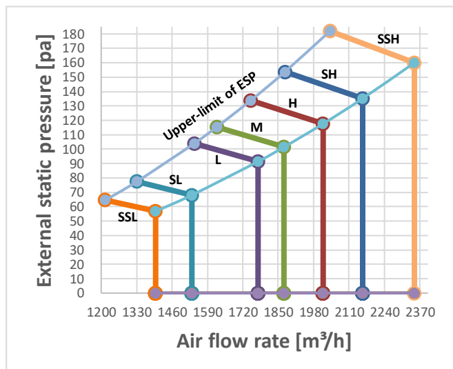
Figure 9.12: MIH160T2HN18
