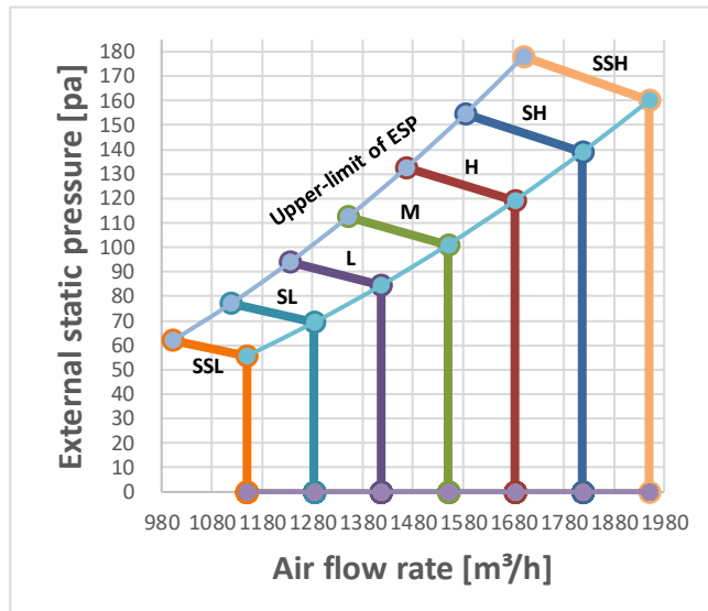
Figure 9.10: MIH112T2HN18
