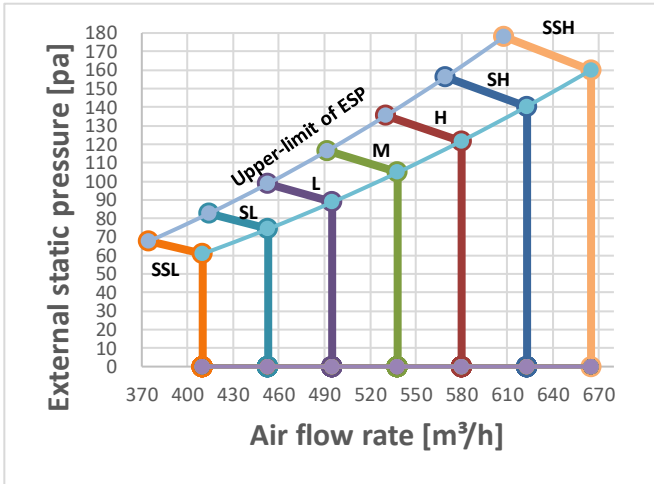
Figure 9.5: MIH45T2HN18
