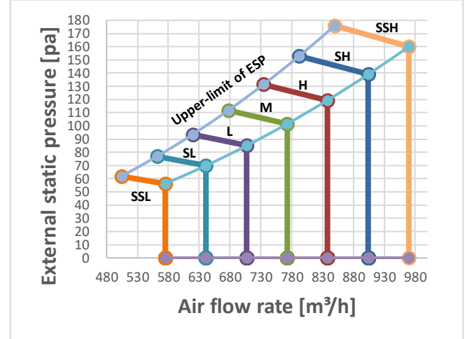
Figure 9.6: MIH56T2HN18
