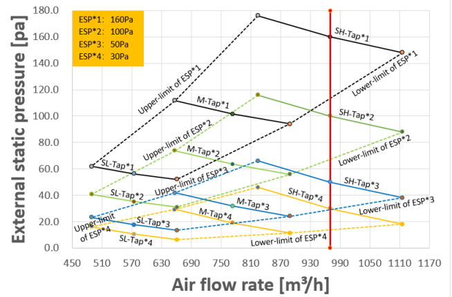
Figure 9.18: MIH56T2HN18
