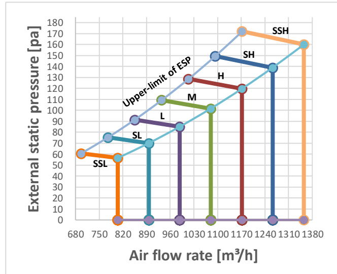
Figure 9.8: MIH80T2HN18
