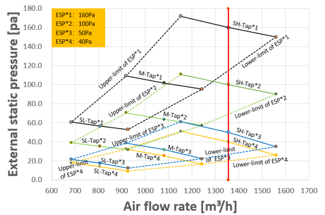
Figure 9.20: MIH80T2HN18
