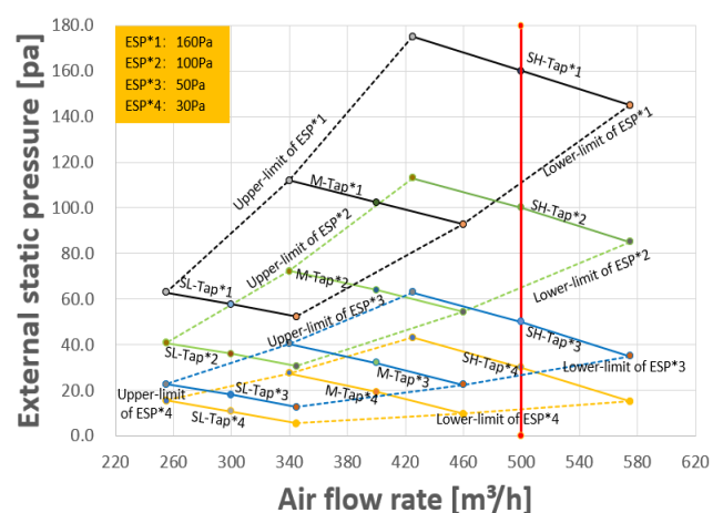
Figure 9.14: MIH22T2HN18
