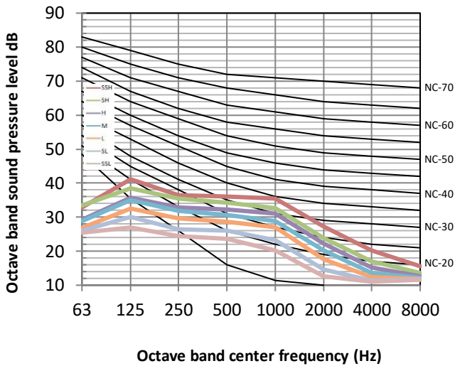
Figure 8.9: MIH71T2HN18 octave band levels
