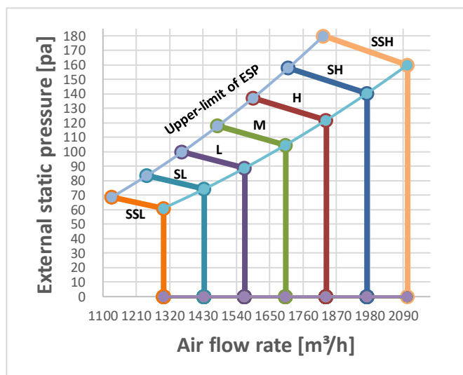
Figure 9.11: MIH140T2HN18
