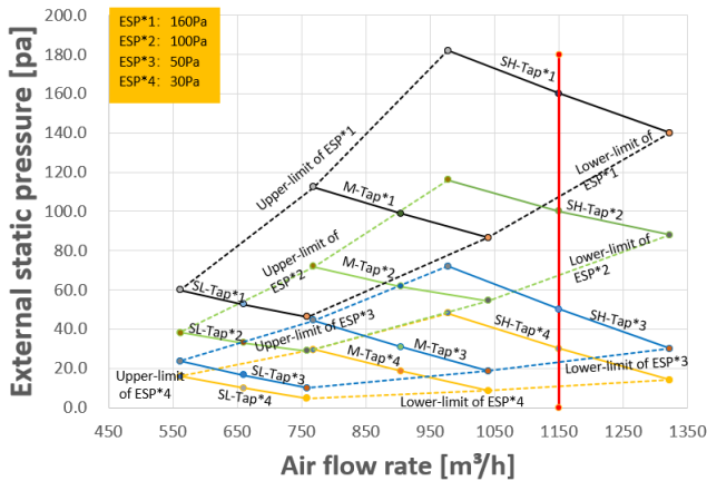
Figure 9.19: MIH71T2HN18
