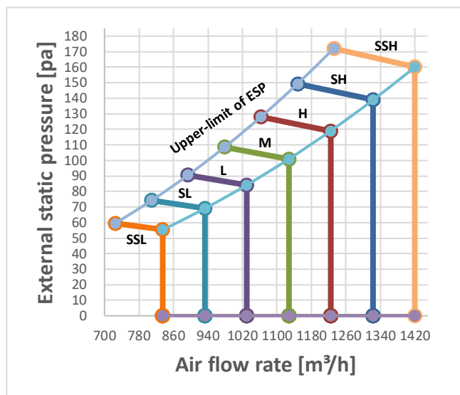
Figure 9.9: MIH90T2HN18
