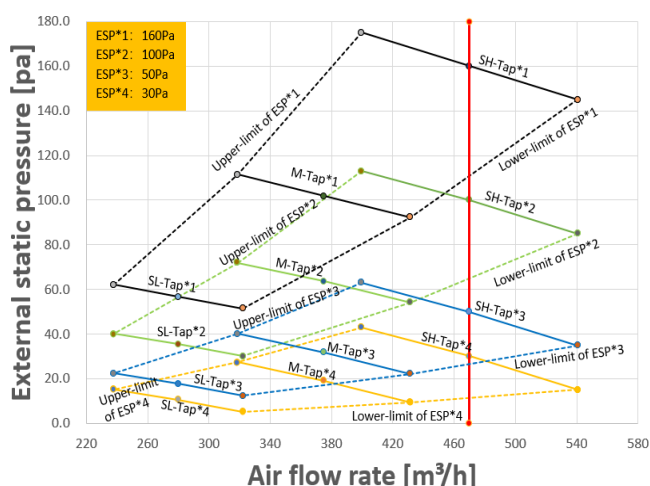
Figure 9.13: MIH15T2HN18
