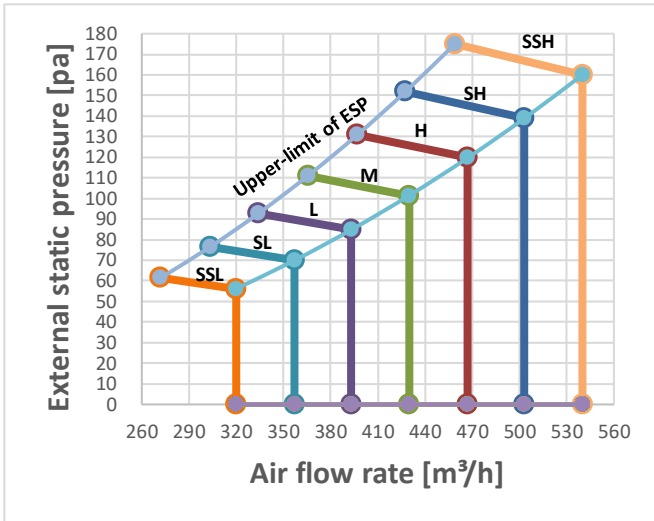
Figure 9.3: MIH28T2HN18
