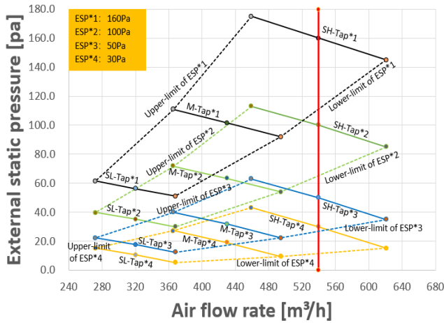
Figure 9.15: MIH28T2HN18
