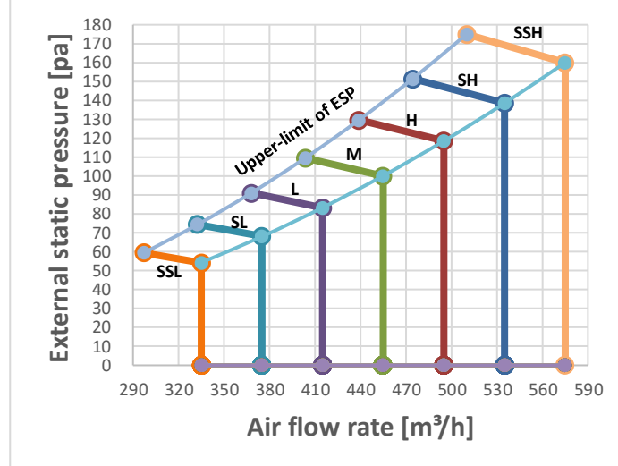
Figure 9.4: MIH36T2HN18
