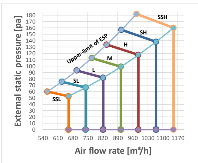
Figure 9.7: MIH71T2HN18
