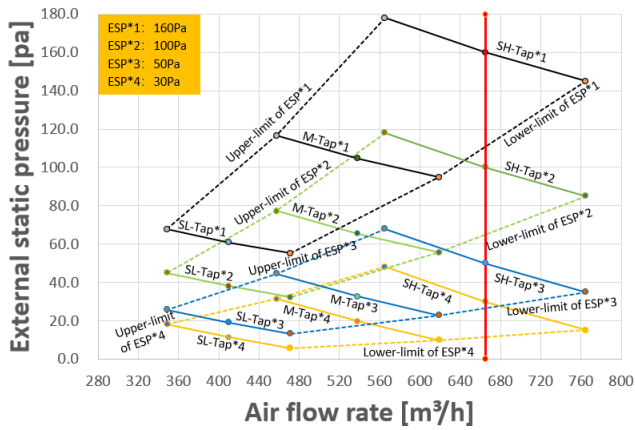
Figure 9.17: MIH45T2HN18
